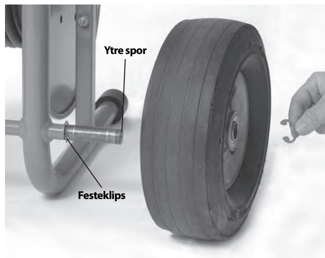
Figur 4 – Montere KJ-2200
