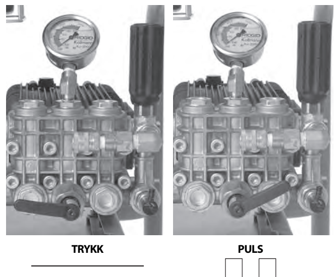
Figur 16 – Stilling for pulsaktuatorspak
