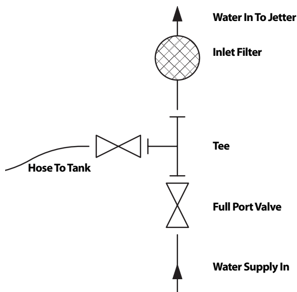
Figure 9 – Water Supply Connections When Using A Tank
