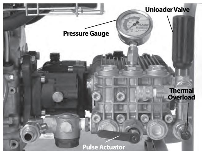
Figure 13 – Controls
